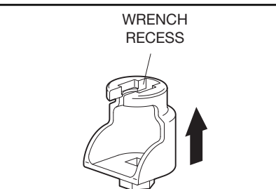
WRENCH RECESS PUSH WRENCH IN TO ENSURE ENGAGEMENT WITH SPRINKLER WRENCHING AREA FIGURE 4 W-TYPE 7 RECESSED SPRINKLER WRENCH
